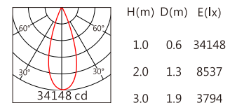
CMU1013 36° 4000K
