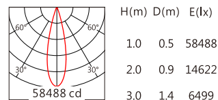
CMU1013 24° 4000K
