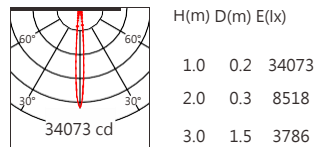
XP-E2 10° 3500K
