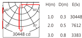
XP-E2 15° 3500K
