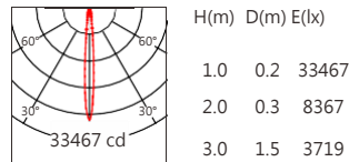
XP-E2 10° 3000K
