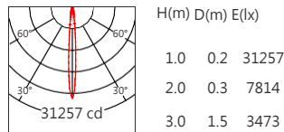
XP-E2 10° 2700K
