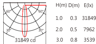
XP-E2 15° 4000K
