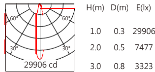
XP-E2 15° 3000K
