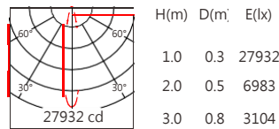
XP-E2 15° 2700K
