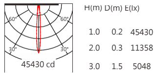
XP-E2 10° 3500K
