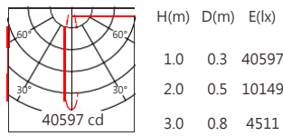
XP-E2 15° 3500K
