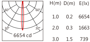
XP-E2 10° 3000K
