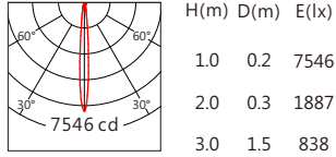
XP-E2 10° 3500K
