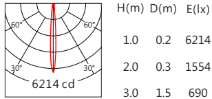
XP-E2 10° 2700K
