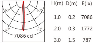
XP-E2 10° 4000K
