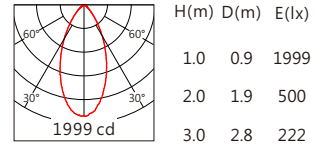
CMU1013 55° 4000K
