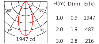
CMU1013 55° 3000K
