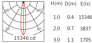
CMU1013 15° 4000K
