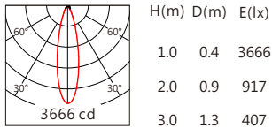
JR-5050 30° 4000K
