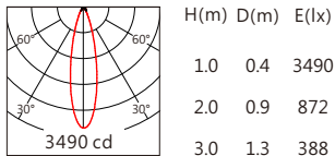
JR-5050 30° 3000K
