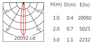
CMB1825 15° 3000K
