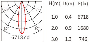
JR-5050 30° 3000K
