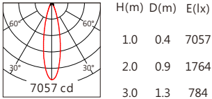
JR-5050 30° 4000K
