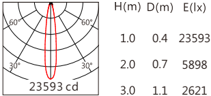
CMB1825 15° 4000K
