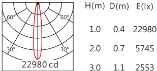
CMB1825 15° 3000K
