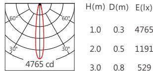
XP-E2 15° 3000K
