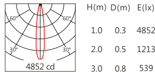
XP-E2 15° 3500K
