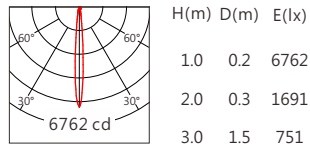
XP-E2 10° 3000K
