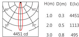
XP-E2 15° 2700K
