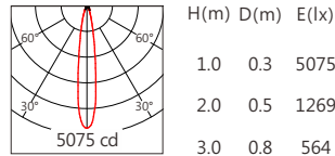
XP-E2 15° 4000K
