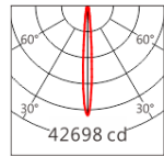
XP-E2 10° 3000K
