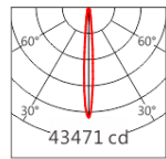
XP-E2 10° 3500K
