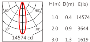
JR-5050 30° 3000K
