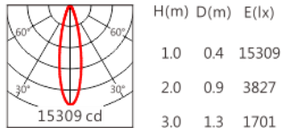
JR-5050 30° 4000K
