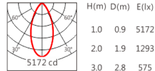
JR-5050 55° 4000K
