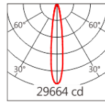
XP-E2 15° 3000K
